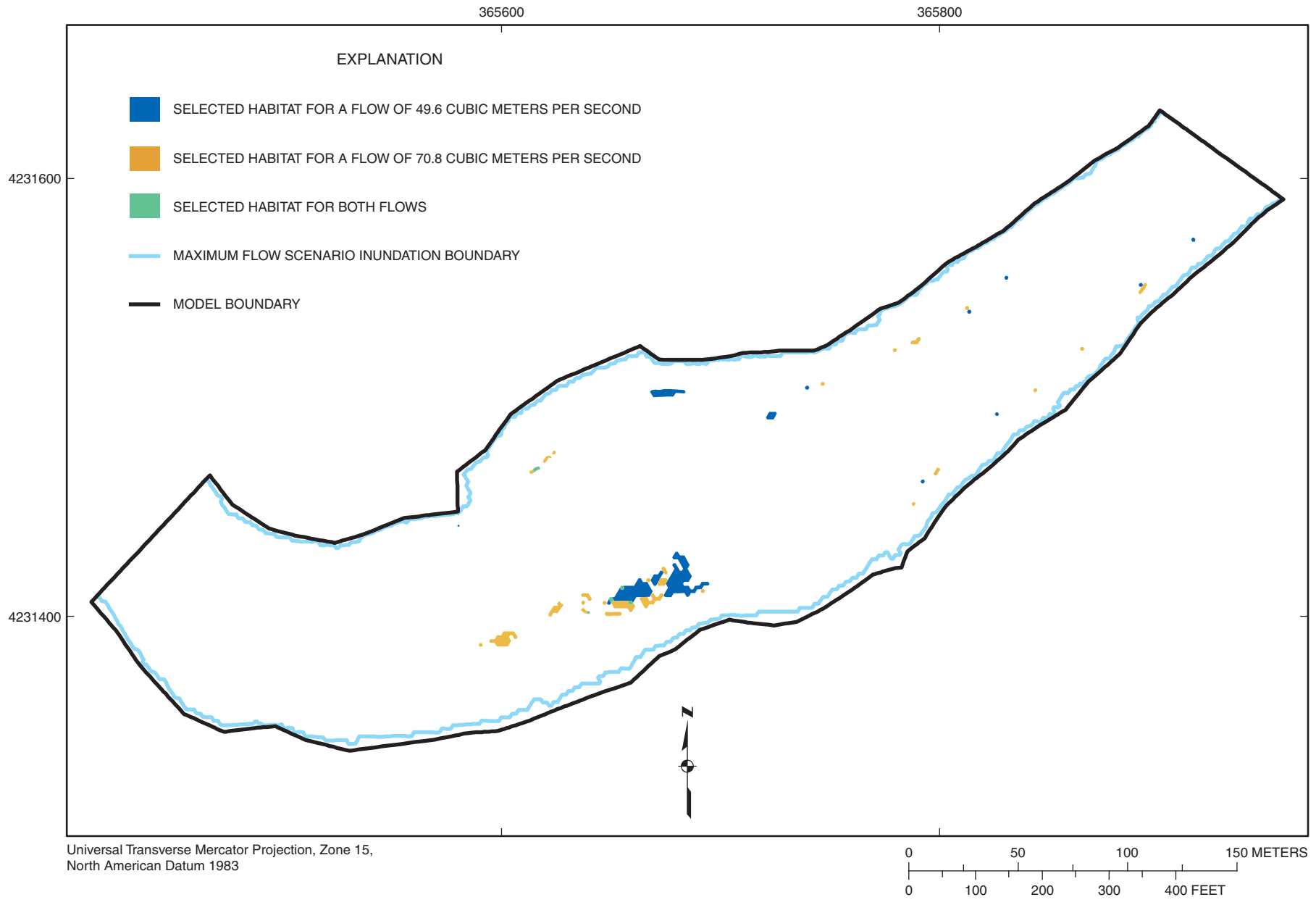
Figure 4-90. Selected habitat area distribution for habitat category 22 (channel catfish) at flows of 49.6 and 70.8 cubic meters per second at Marais des Cygnes River site MDC2.
